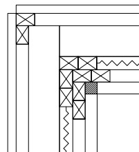
Figure 8b. View from top
