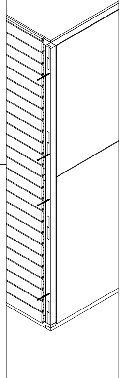
Figure 2.2b. Corner fixing
