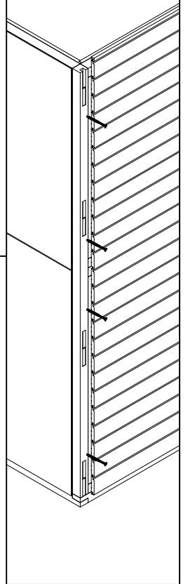
Figure 2.1b. Corner fixing
