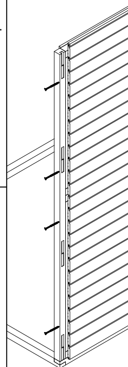
Figure 2b. Corner fixing
