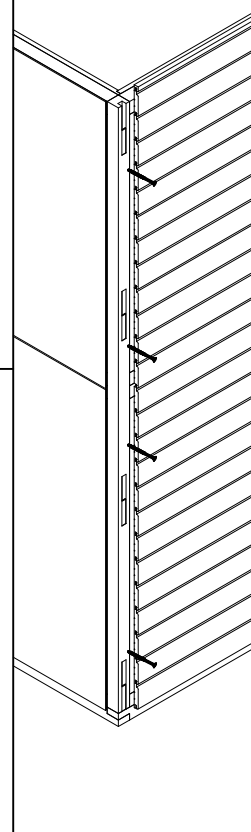
Figure 2.1b. Corner fixing
