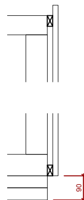
Exterior cladding (side view)
